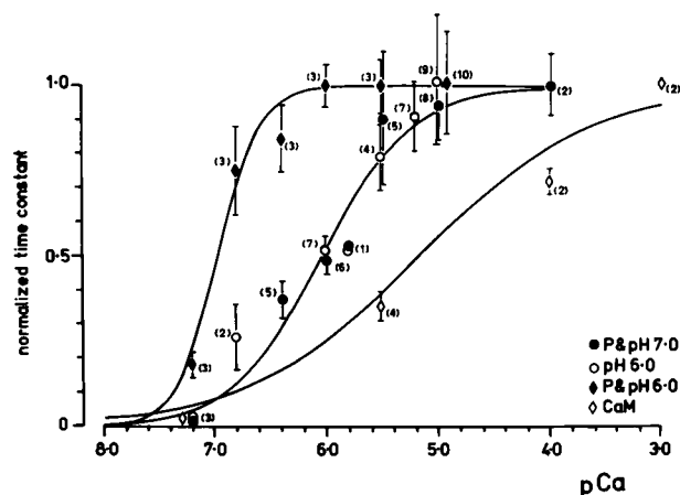
FIGURE 4 Normalized time constants of the decrease in junctional conductance elicited by perfusion solutions of different calcium concentrations. In each of the three series of experiments, each experiment at one pCa value was fitted to an exponential curve, and the time constants calculated and averaged. These were normalized with respect to the maximal rate of decrease in conductance (smallest time constant) within the series. The reciprocal of this value was then plotted against the calcium concentration. Calmodulin (CaM) data was analyzed similarly. Data points are plotted as mean \pm SE. Solid circles represent the effect of the phosphorylating cocktail buffered at pH 7.0, whereas open circles show the effect of pH 6. Both sets of data points fell on the same curve, with a K_{0.5} of 0.94 \mu M. Solid diamonds show the effect of the phosphorylating cocktail buffered at pH 6.0 and open diamonds show data obtained with CaM (10 \mu M) in the perfusing solution (15). The K_{0.5} 's are 0.1 and 7.4 \mu M, respectively. The number of experiments performed at each pCa is shown between parenthesis. The data points have been fitted to a curve of the type y = 1/(1 + \exp[(pCa - pK_{0.5})k]) , where pK_{0.5} is the half maximal pCa and k is the slope at half maximal response. The value of k for the curves that fit the data points for the phosphorylating cocktail at pH 7.0, and low pH, is \sim 0.5 .
